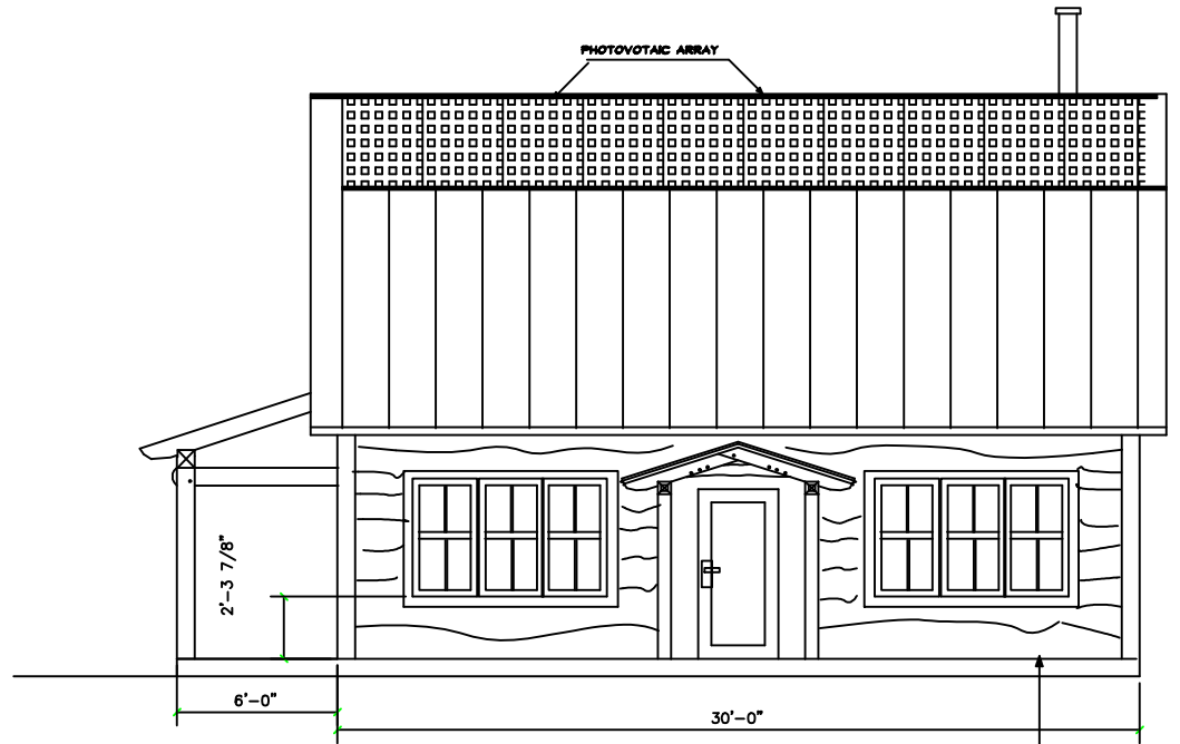
SOUTH ELEVATION
