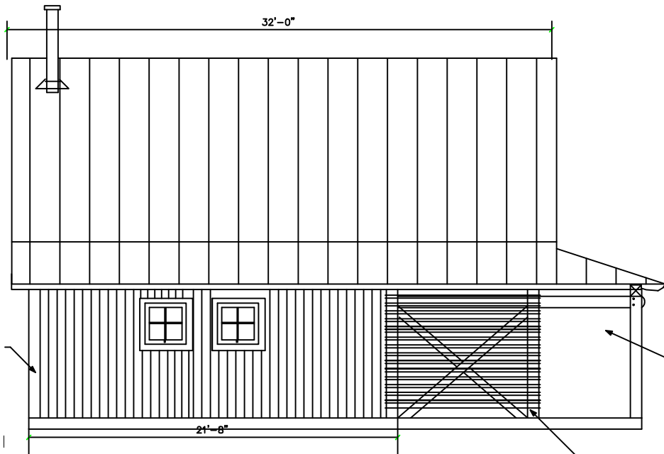
NORTH ELEVATION
